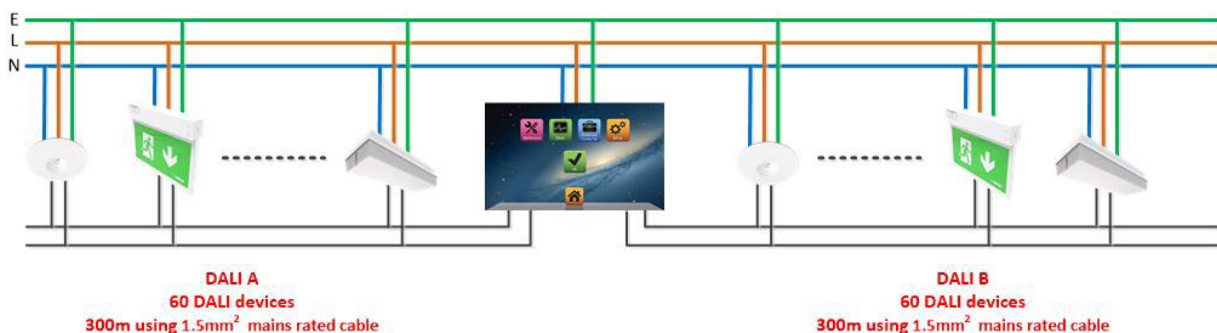
Wiring Diagram – Self-Contained emergency operation
