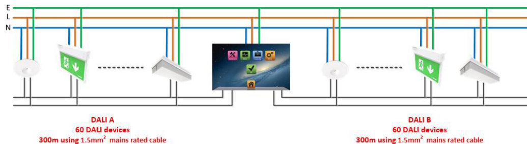
Wiring Diagram – Self-Contained emergency operation
