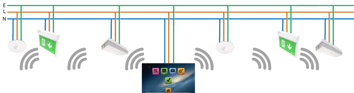
Wiring Diagram – Self-Contained emergency operation
