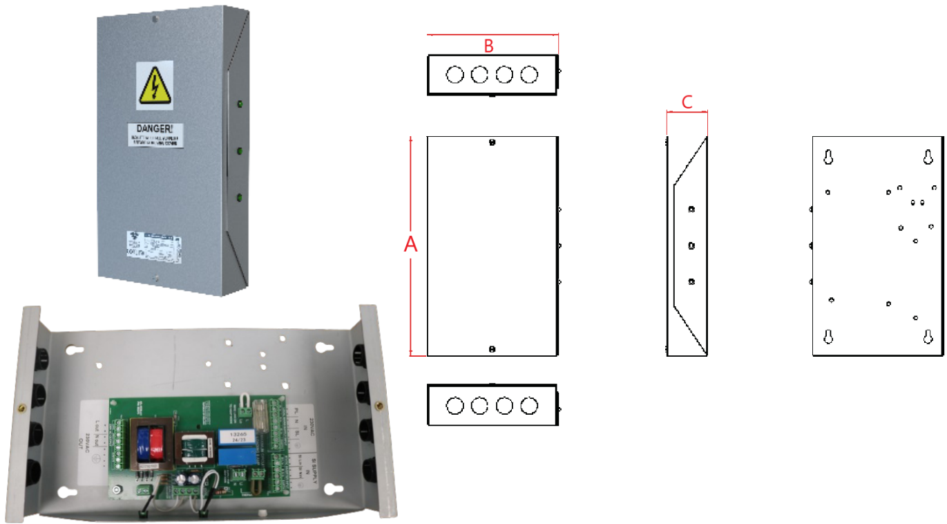
Example of SICOU1/SCM1 Model
